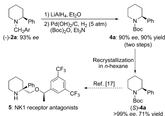
Scheme 2. The formal synthesis of NK1 receptor antagonist 5 . Boc = tert -butoxyloxycarbonyl.
